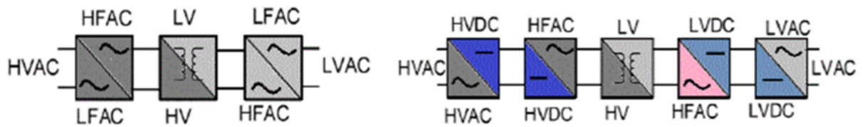
Figure 1: Different Block Diagrams for SSTs 4
