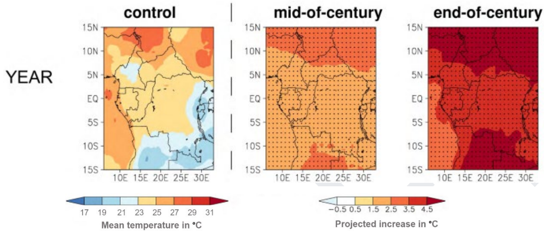
Figure 4: Maps of projected changes for mean temperature under a high emission scenario. Stippled areas indicate "robust" changes where 66 percent of all models project a climate change signal in the same direction. Source: CSC 2013
