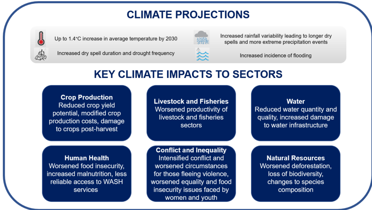
Figure 2. Summary of climate projections and key climate impacts to resilience and food security program areas.
