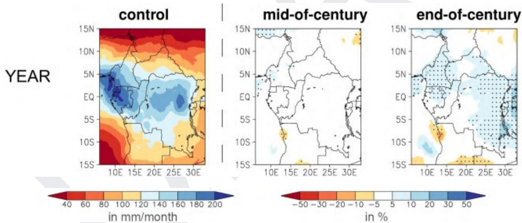
Figure 5: Maps of projected changes for total precipitation under a high emission scenario. Stippled areas indicate "robust" changes where 66 percent of all models project a climate change signal in the same direction. Source: CSC 2013
