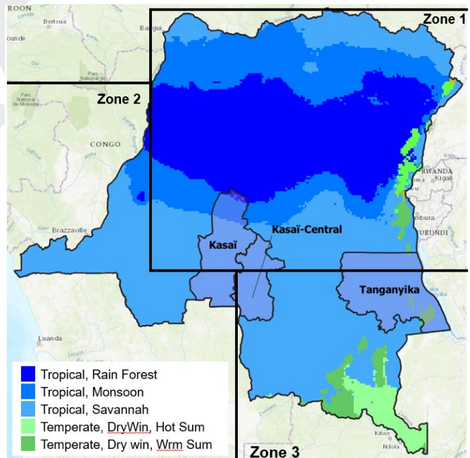
Figure 3: Climate zones and Koepfen-Geiger climate classification of the DRC, overlaying provinces of interest. Climate zones are from the Climate Service Center (CSC)'s Climate Change Scenarios for the Congo Basin.
